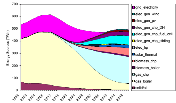
Figure 4 Energy supplied from a range of sources out to 2050 (Scenario C)
