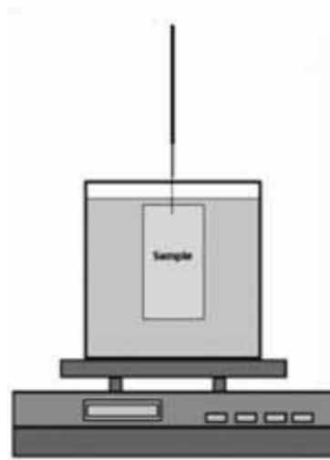
Figure 7: Diagram of water displacement method for measuring wood core volume. The core is forced underwater with a needle. The core should not touch the edges of the container. When the sample is sunk underwater, the level of water raises, and, for the balance everything is as if one had added the amount of water equivalent to the volume of the sample. Therefore the reading on the digital balance is equal to the volume of the core (with the equivalence 1 g = 1 cm 3 ).
